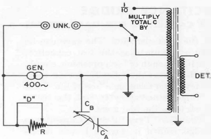
Figure 2. Basic bridge circuit.
