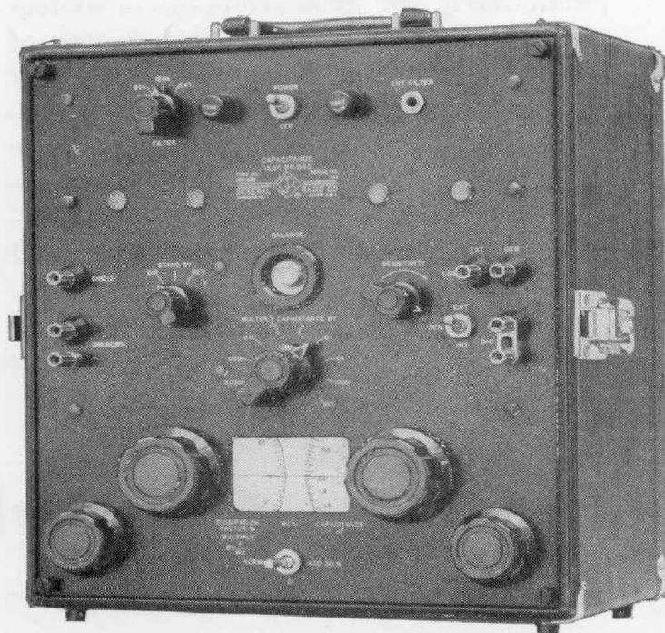
Figure 1. Panel view of Type 1611-B Capacitance Test Bridge.
