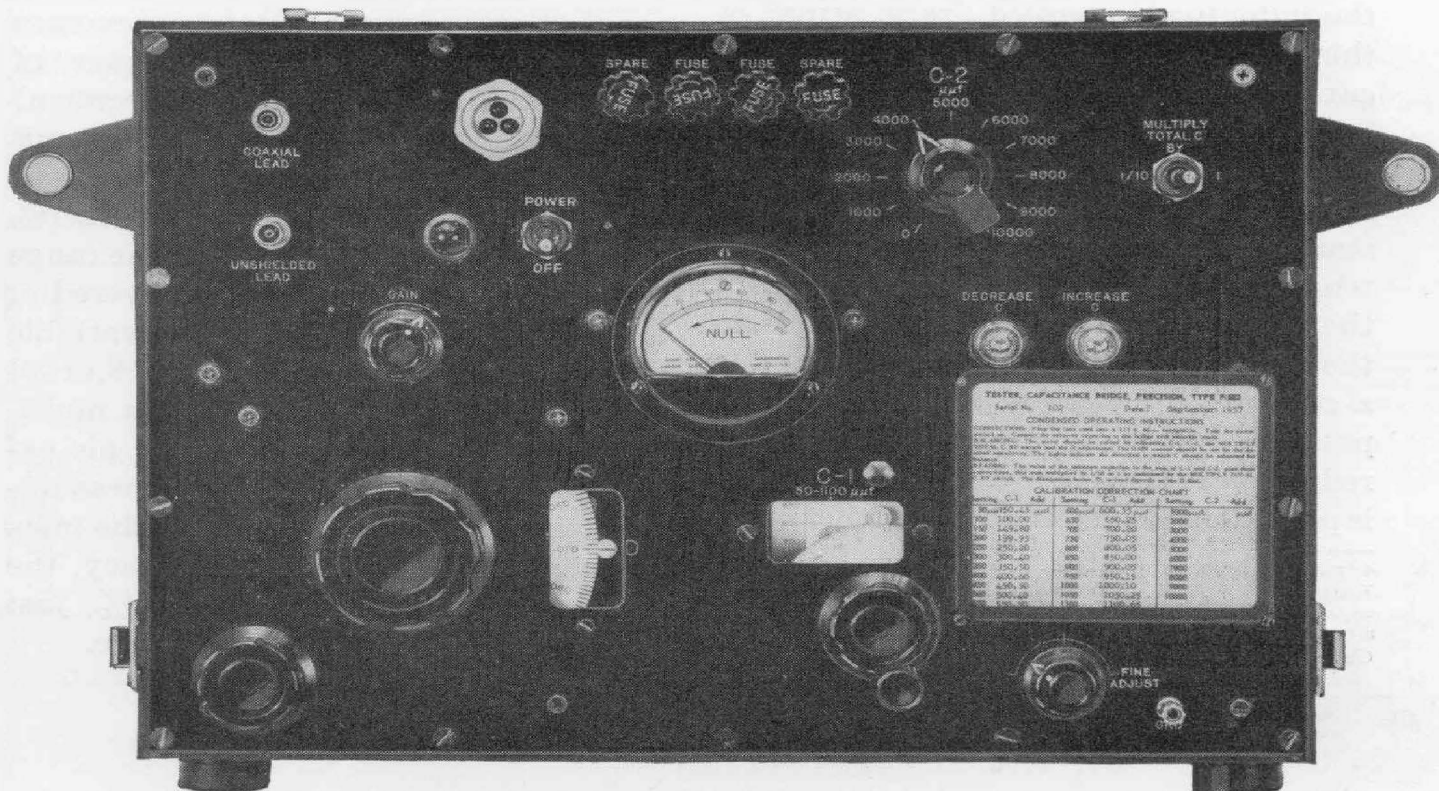
Figure 1. Panel view of the Type P-582 Capacitance Bridge.
