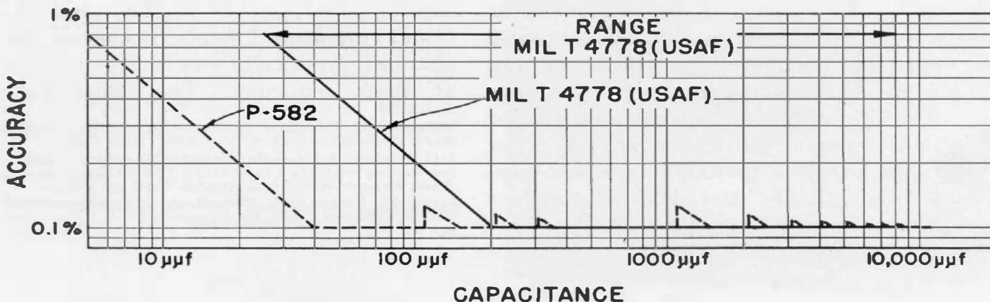
Figure 3. Plot of percentage accuracy versus capacitance measured.
